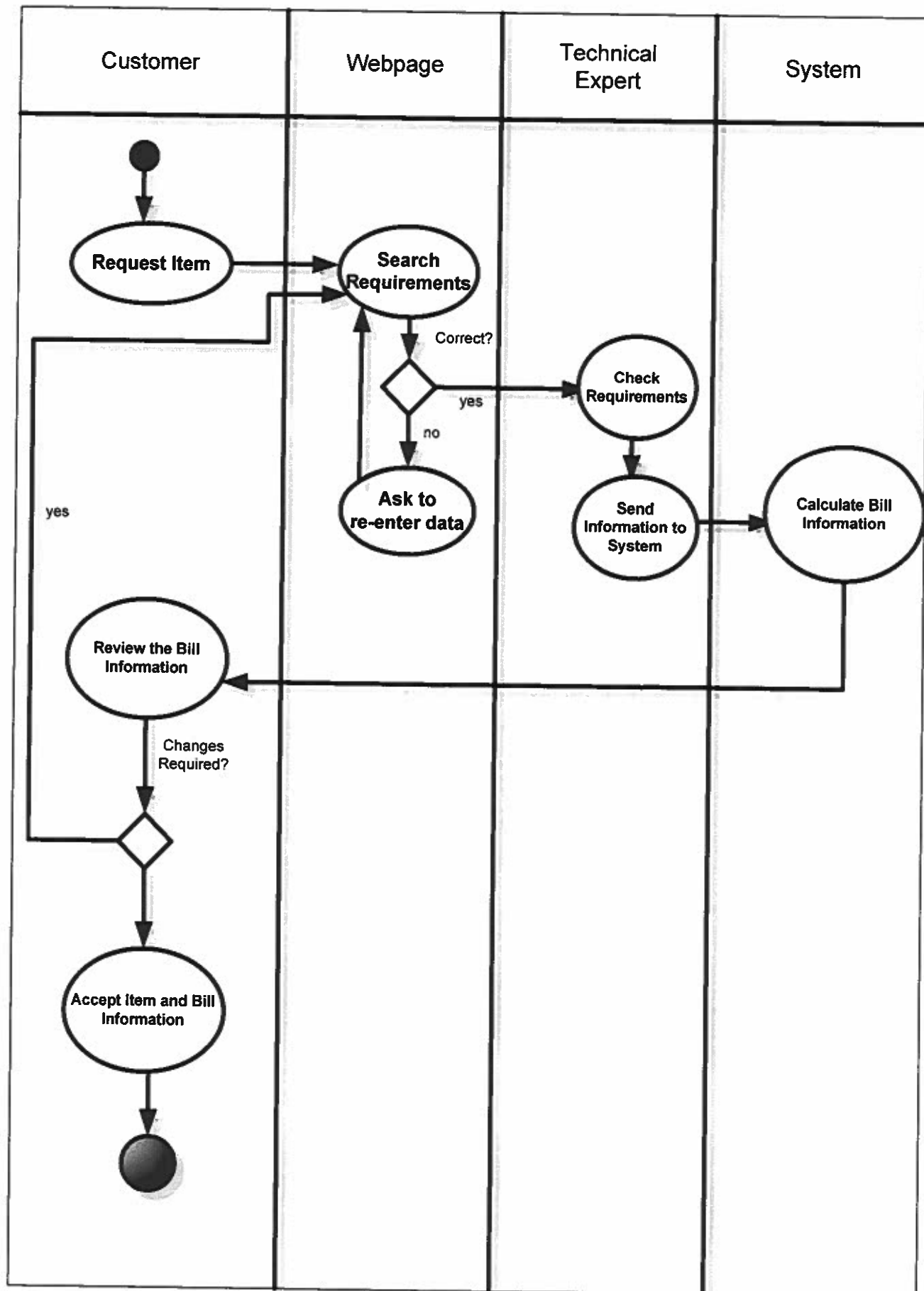
Activity Diagram
